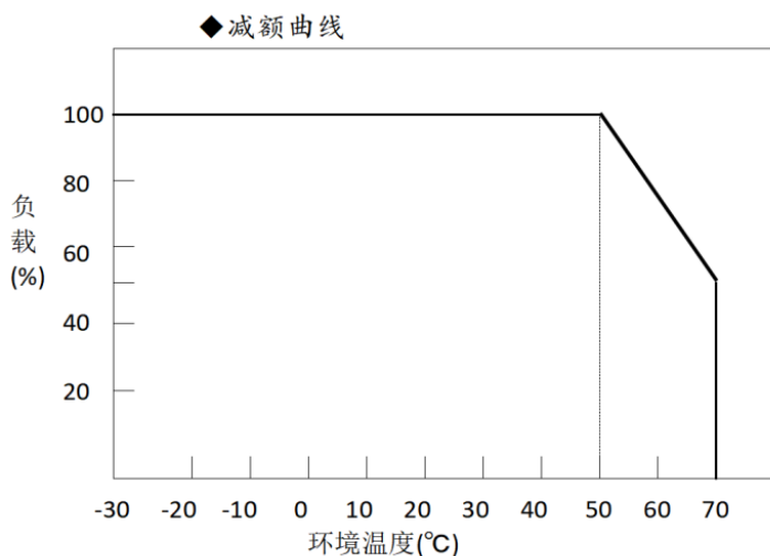
■ 降额曲线 Derating Curve
