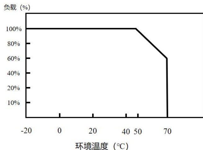
■ 降额曲线 Derating Curve
