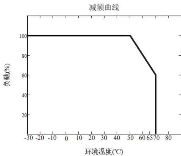
■ 降额曲线 Derating Curve
