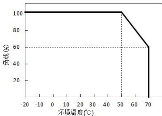
■ 降额曲线 Derating Curve
